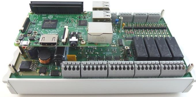
Figure 14: Assembled DIN rail housing
