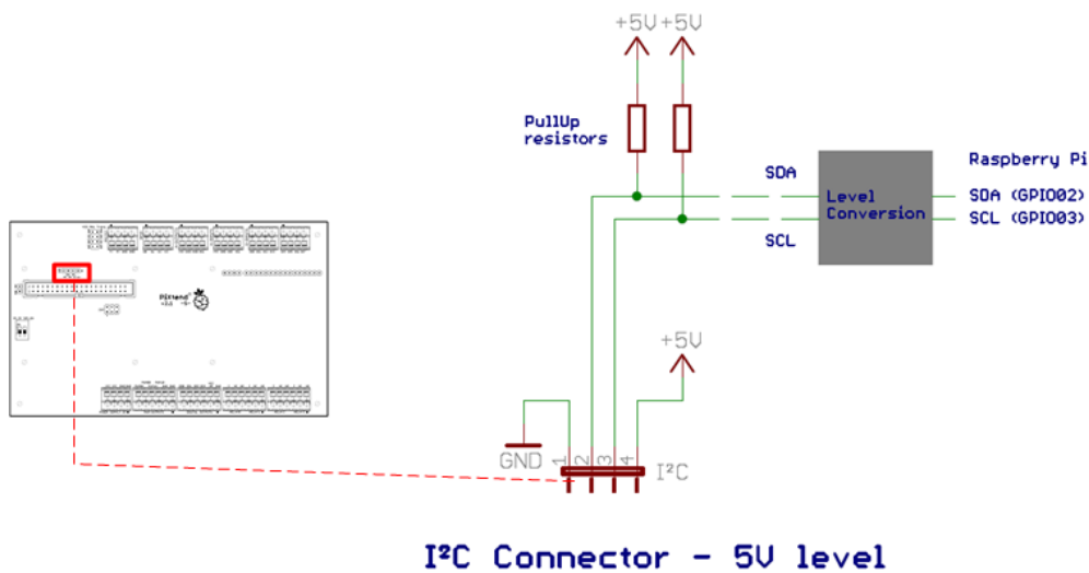
Figure 44: Simplified wiring diagram: I²C at 5V level
